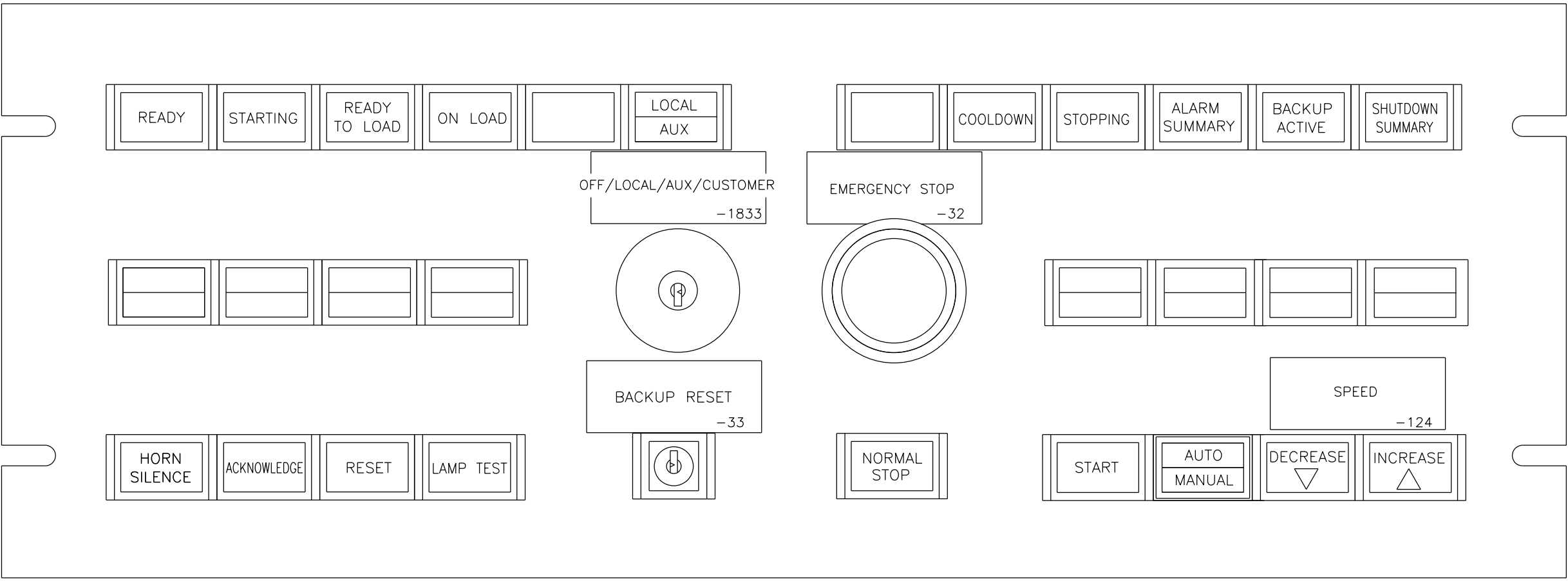
FRONT VIEW
